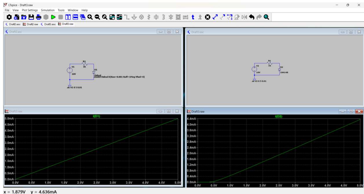
Figure 3: DC sweep for Ideal and 1N4148 diodes
